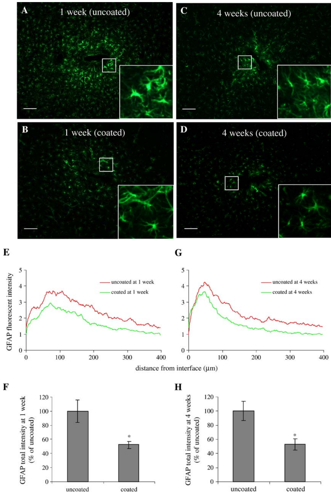
Fig. 2 – (A–D) Representative images of GFAP staining for astrocytes in the horizontal brain sections 1 week and 4 weeks post implantation for both uncoated and DEX-coated probes. Scale bar = 100 \mu\text{m} . Inset denotes higher magnification (fourfold) of identified area showing the morphology of reactive astrocytes. (E, G) GFAP fluorescent intensity profiles as a function of distance 1 week and 4 weeks post implantation. (F, H) Quantification of total GFAP fluorescent intensity 1 week and 4 weeks post implantation ( n=4 ). * P<0.05 compared with uncoated probes.
