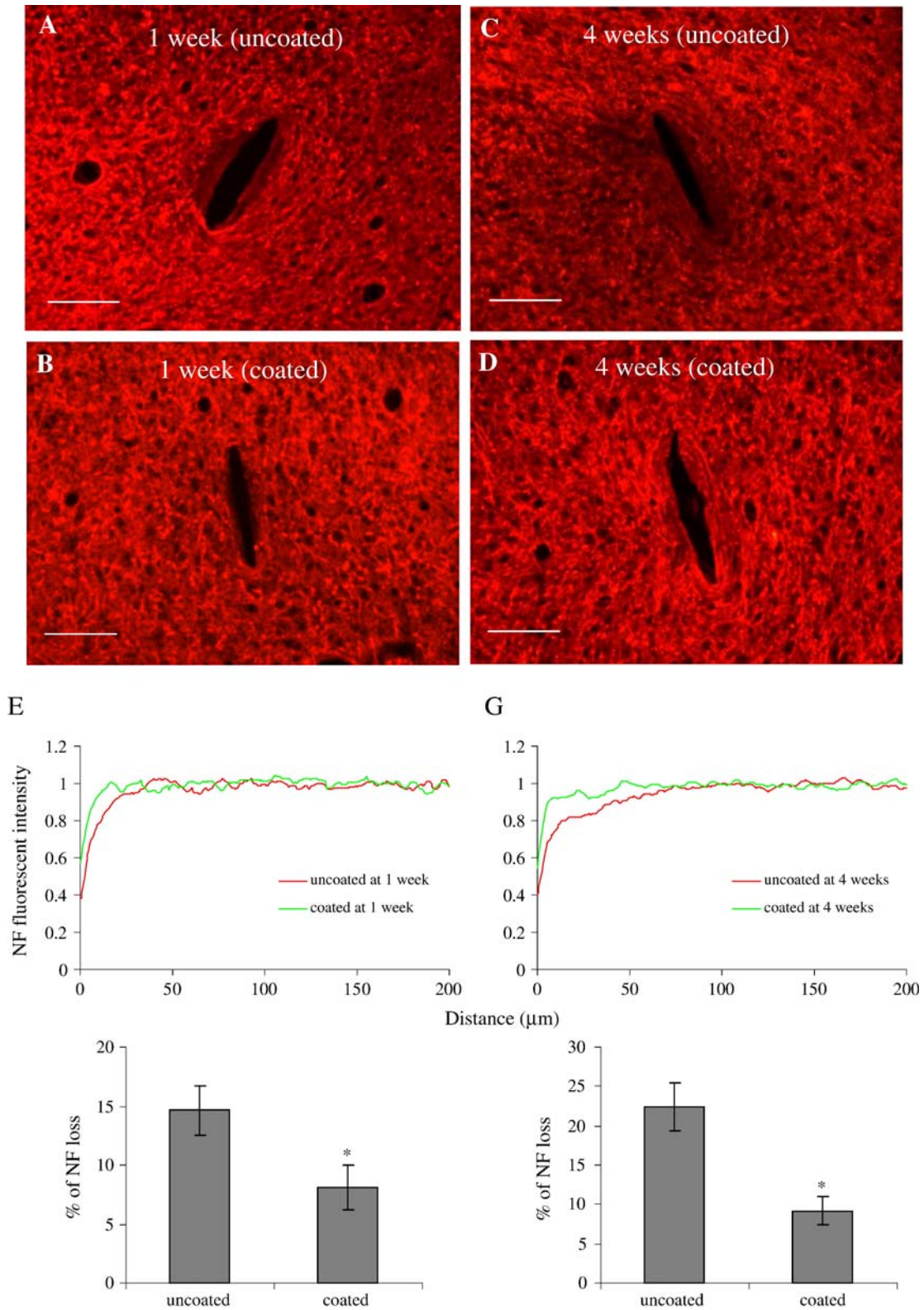
Fig. 6 - (A-D) Representative images of NF160 staining for neurons in the horizontal brain sections 1 week and 4 weeks post implantation for both uncoated and DEX-coated probes. Scale bar=100 μm. (E, G) NF fluorescent intensity profiles as a function of distance 1 week and 4 weeks post implantation. (F, H) Quantification of % NF loss 1 week and 4 weeks post implantation ( n=4 ). * P<0.05 compared with uncoated probes.
