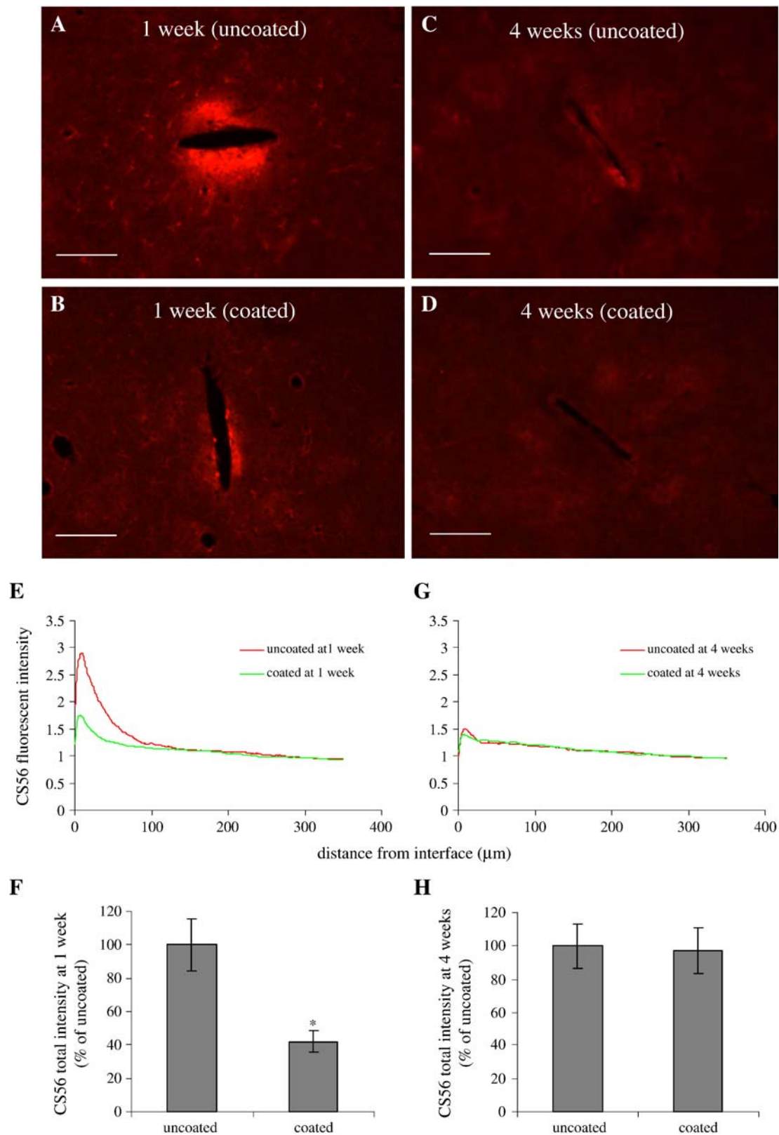
Fig. 3 – (A–D) Representative images of CS56 staining for GSPGs in the horizontal brain sections 1 week and 4 weeks post implantation for both uncoated and DEX-coated probes. Scale bar=100 \mu\text{m} . (E, G) CS56 fluorescent intensity profiles as a function of distance 1 week and 4 weeks post implantation. (F, H) Quantification of total CS56 fluorescent intensity 1 week and 4 weeks post implantation ( n=4 ). * P<0.05 compared with uncoated probes.
