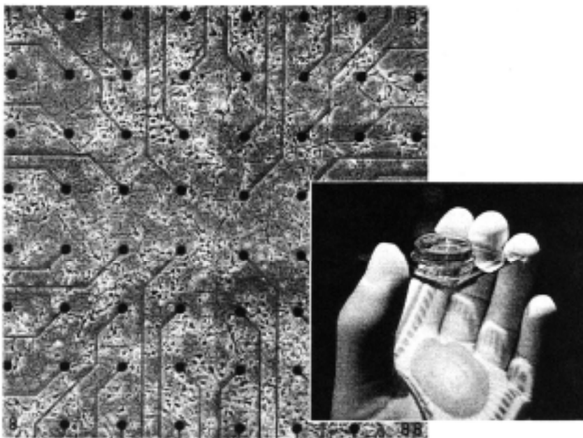
Fig. 1. 60-electrode MEA from MultiChannel Systems, with devolving rat cortical culture after 6 days in vitro. The 10- \mu\text{m} diam. electrodes (not visible in the center of a 30- \mu\text{m} gold disk) are 200 \mu\text{m} apart, with sputtered titanium nitride to reduce impedance. The gold leads (beneath an insulating layer of silicon nitride) travel under a glass ring, containing cell culture medium, to contacts around the perimeter of the 50-mm glass plate (inset). These are connected to preamplifiers, analog-to-digital converters, and to a computer. They can also be connected to stimulation circuitry, allowing long-term two-way communication between the neurons growing over the electrodes and the computer.
